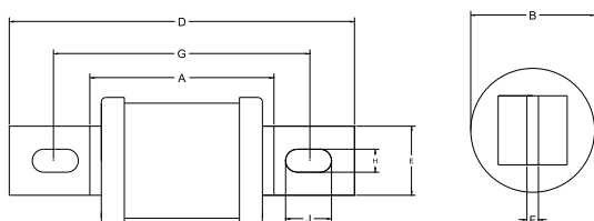
BS88: Part 2 reference 'B' fuse-link dimensions and tag variants
