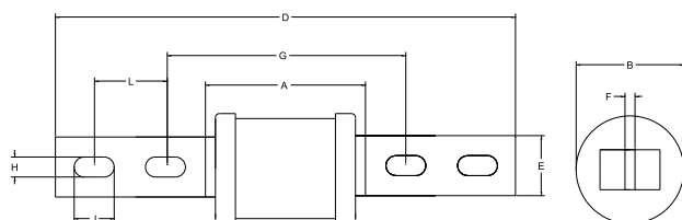
BS88: Part 2 reference 'C' fuse-link dimensions and tag variants
