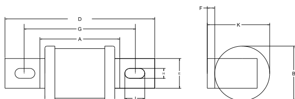
BS88: Part 2 reference 'A' fuse-link dimensions and tag variants
