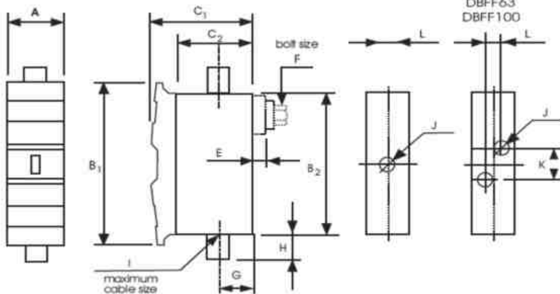
TYPES DBFF20A1, DBFF32, DBFF63, DBFF100
